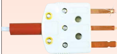
Miniature Connector, MTP-U-M (Add £4.70), (e.g., RTD-2-F3105-1M-T-MTP).
