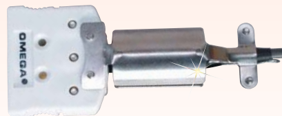
4 to 20 mA Transmitter, SPRTX (Add £50) [e.g., RTD-2-F3105-1M-G-SPRTX(M1)].
